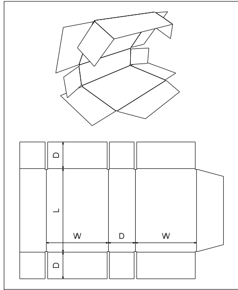
FEFCO\0400 - Folder Type Boxes\ FEFCO 0410
