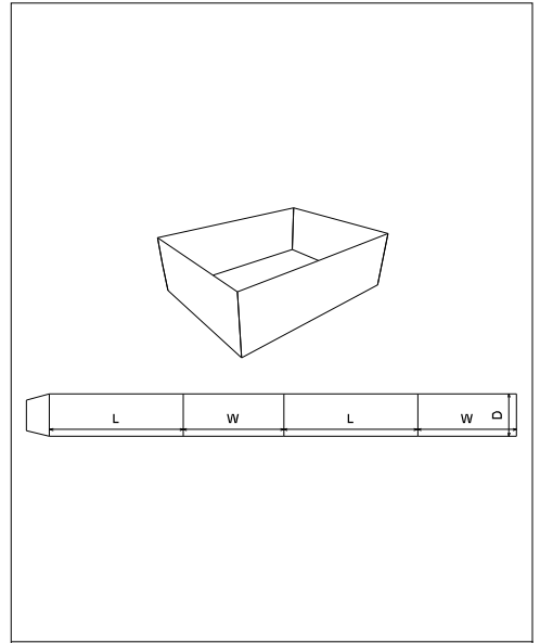
FEFCO\0500 - Slide Type Boxes\ FEFCO 0501
