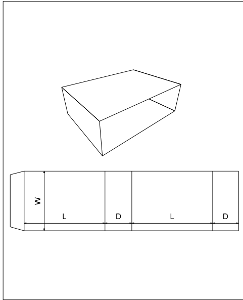
FEFCO\0500 - Slide Type Boxes\ FEFCO 0502
