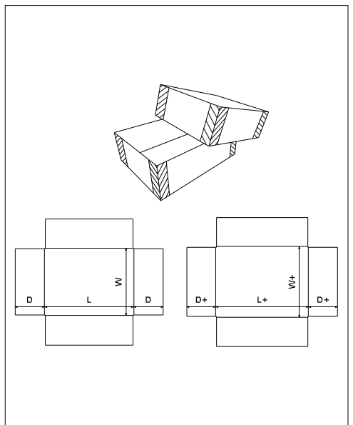
FEFCO\0300 - Telescope Type Box\ FEFCO 0302
