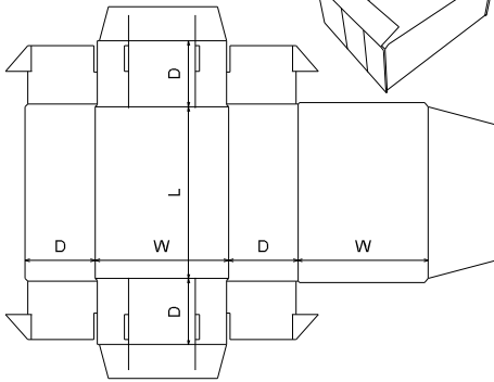
FEFCO\0400 - Folder Type Boxes\ FEFCO 0445
