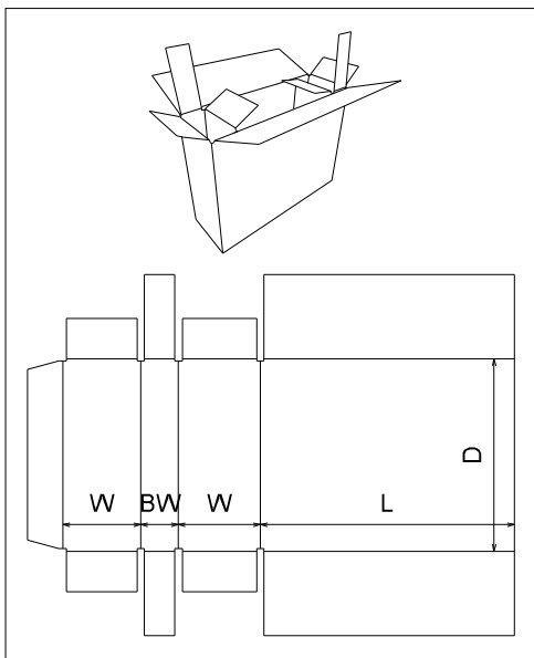
FEFCO\0600 - Rigid Type Boxes\ FEFCO 0621
