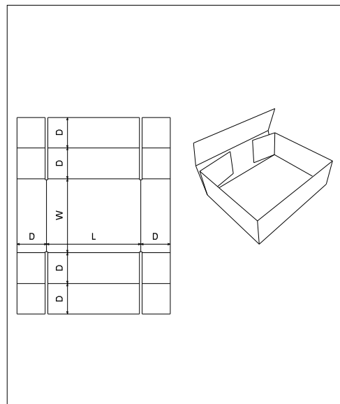
FEFCO\0400 - Folder Type Boxes\ FEFCO 0455
