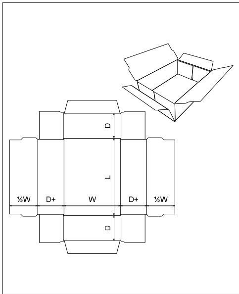
FEFCO\0400 - Folder Type Boxes\ FEFCO 0415
