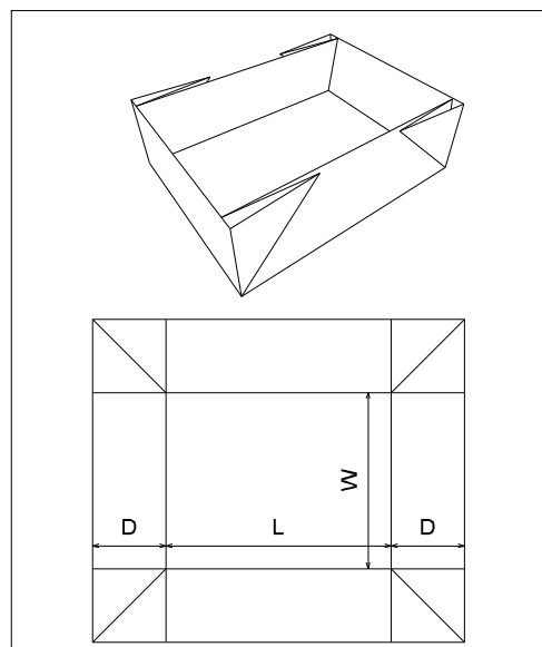
FEFCO\0400 - Folder Type Boxes\ FEFCO 0449
