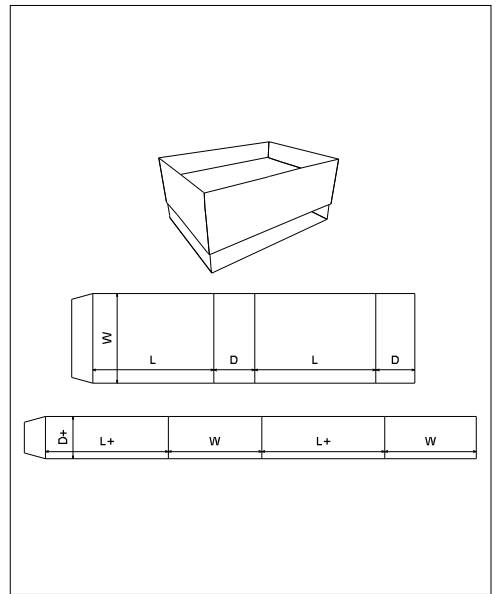
FEFCO\0500 - Slide Type Boxes\ FEFCO 0504
