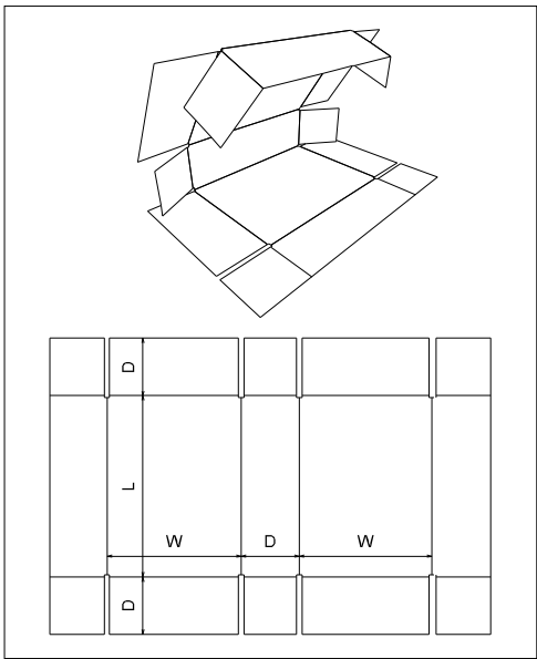
FEFCO\0400 - Folder Type Boxes\ FEFCO 0409
