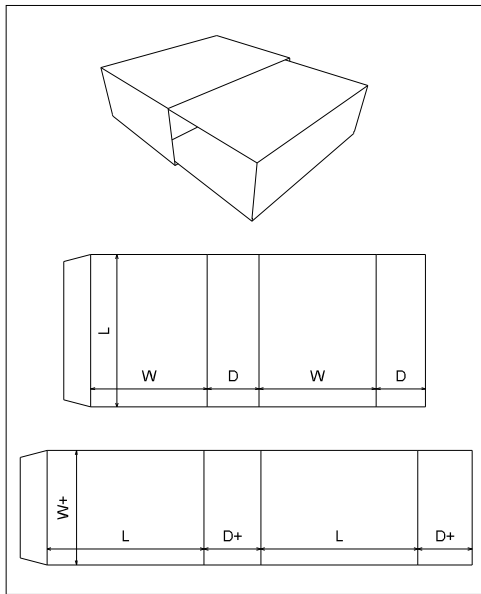
FEFCO\0500 - Slide Type Boxes\ FEFCO 0505
