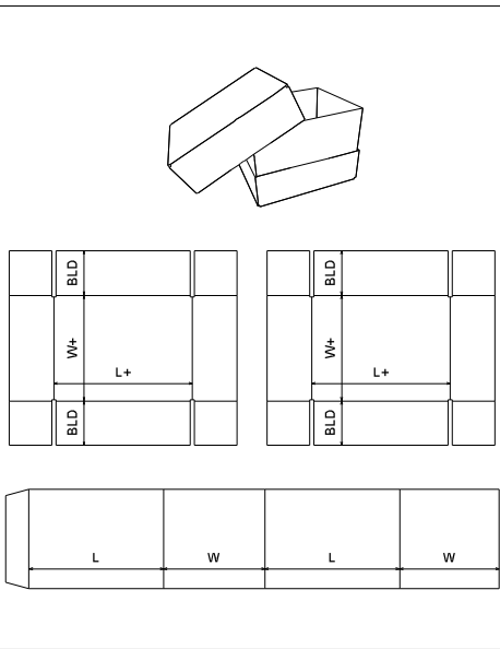
FEFCO\0300 - Telescope Type Box\ FEFCO 0310
