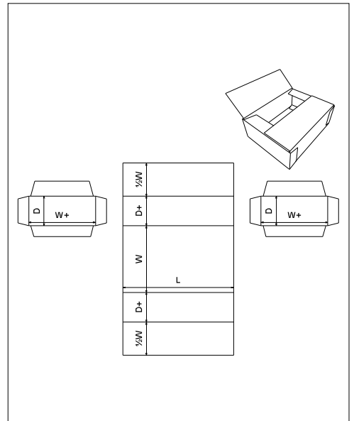
FEFCO\0600 - Rigid Type Boxes\ FEFCO 0605
