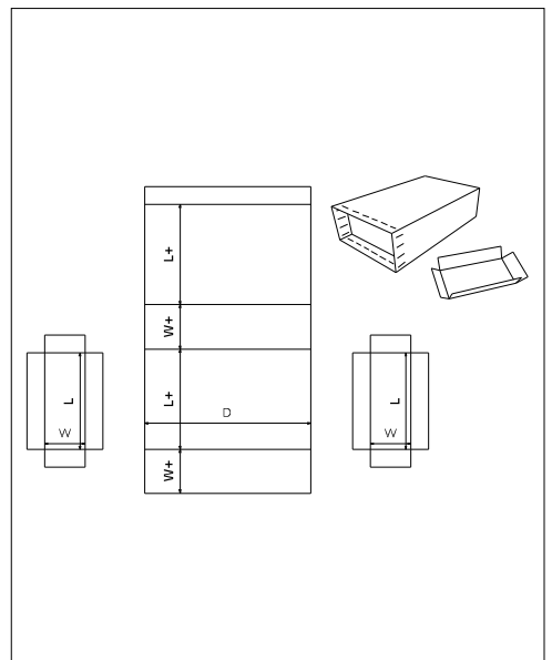
FEFCO\0600 - Rigid Type Boxes\ FEFCO 0616
