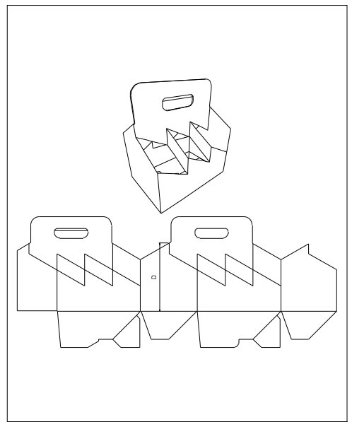
FEFCO\0700 - Ready Glued Cases\ FEFCO 0717 - Bottle Carrier
