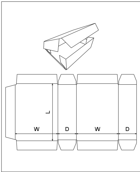
FEFCO\0400 - Folder Type Boxes\ FEFCO 0406
