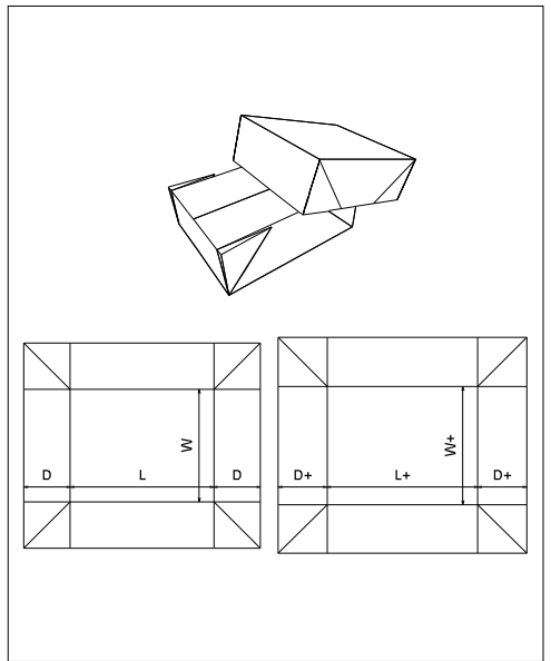
FEFCO\0300 - Telescope Type Box\ FEFCO 0309
