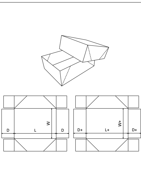
FEFCO\0300 - Telescope Type Box\ FEFCO 0303
