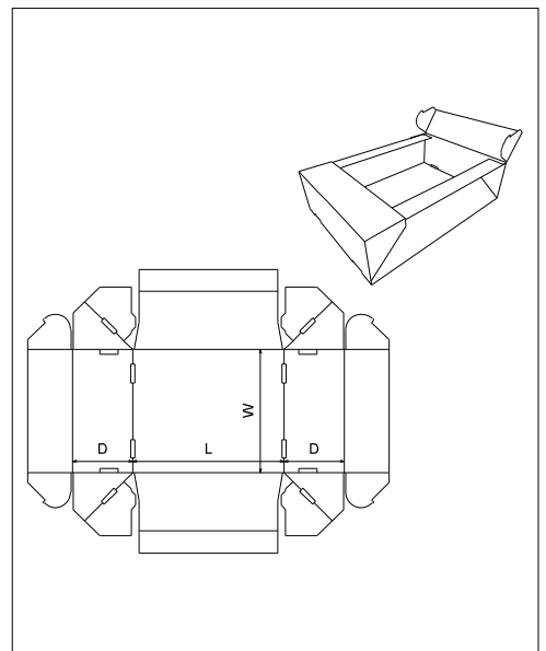
FEFCO\0700 - Ready Glued Cases\ FEFCO 0773
