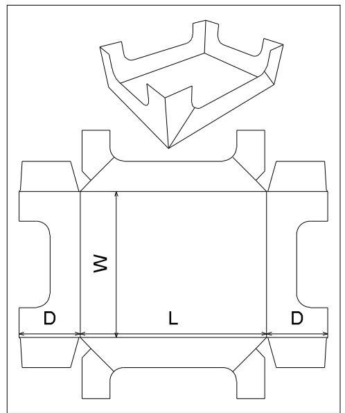
FEFCO\0700 - Ready Glued Cases\ FEFCO 0770
