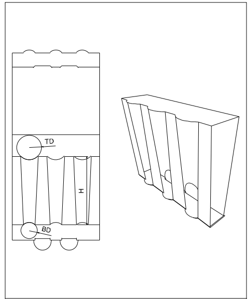
FEFCO\0700 - Ready Glued Cases\ FEFCO 0752 - Glass Pack
