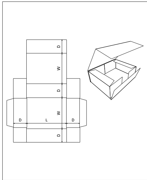
FEFCO\0400 - Folder Type Boxes\ FEFCO 0413
