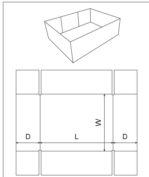
FEFCO\0400 - Folder Type Boxes\ FEFCO 0452
