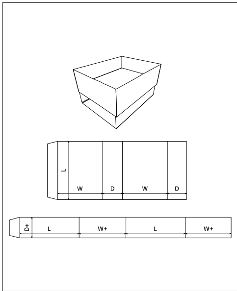
FEFCO\0500 - Slide Type Boxes\ FEFCO 0507
