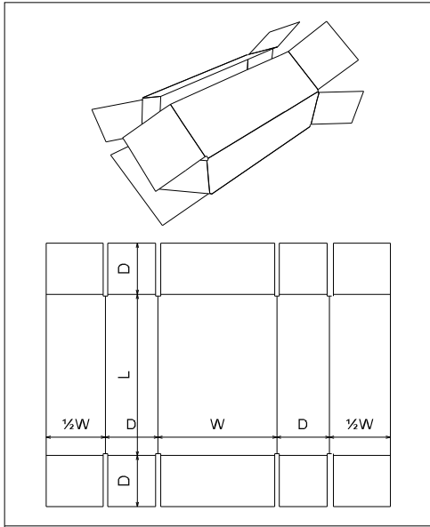
FEFCO\0400 - Folder Type Boxes\ FEFCO 0411
