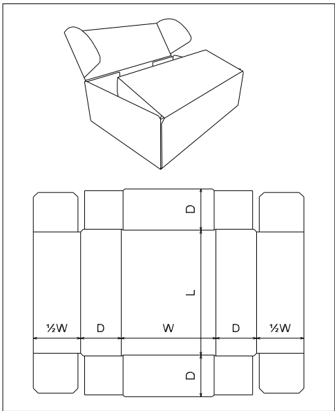
FEFCO\0400 - Folder Type Boxes\ FEFCO 0416
