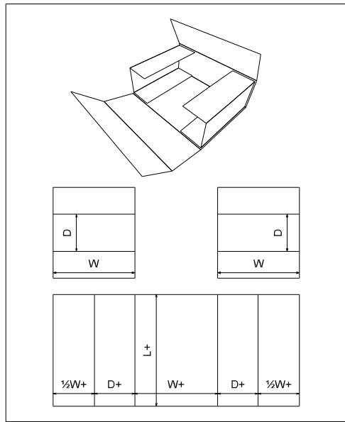
FEFCO\0400 - Folder Type Boxes\ FEFCO 0405
