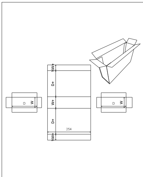
FEFCO\0600 - Rigid Type Boxes\ FEFCO 0620
