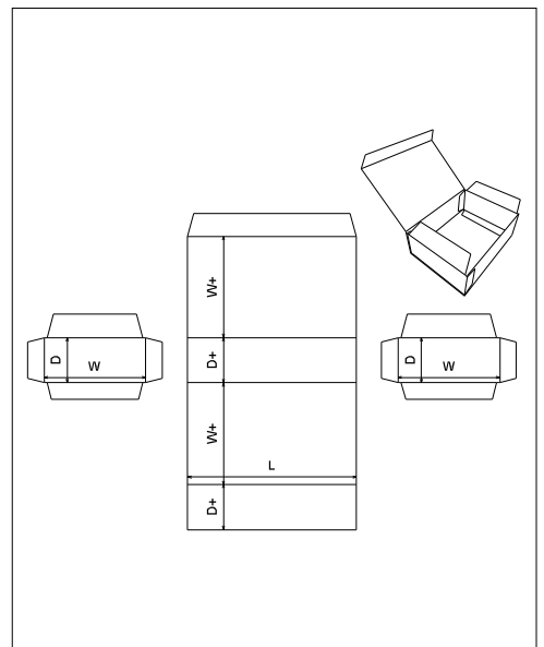
FEFCO\0600 - Rigid Type Boxes\ FEFCO 0608
