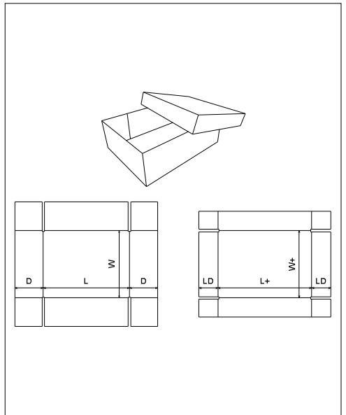
FEFCO\0300 - Telescope Type Box\ FEFCO 0306
